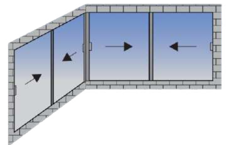
Corner Sliding System
